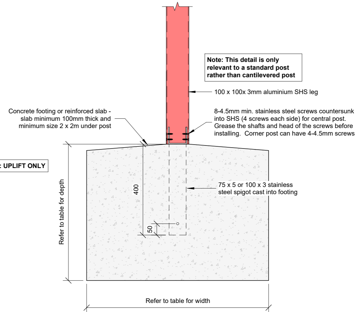
LOUVRE STANDARD POST BASE CONNECTION 1 : 10
