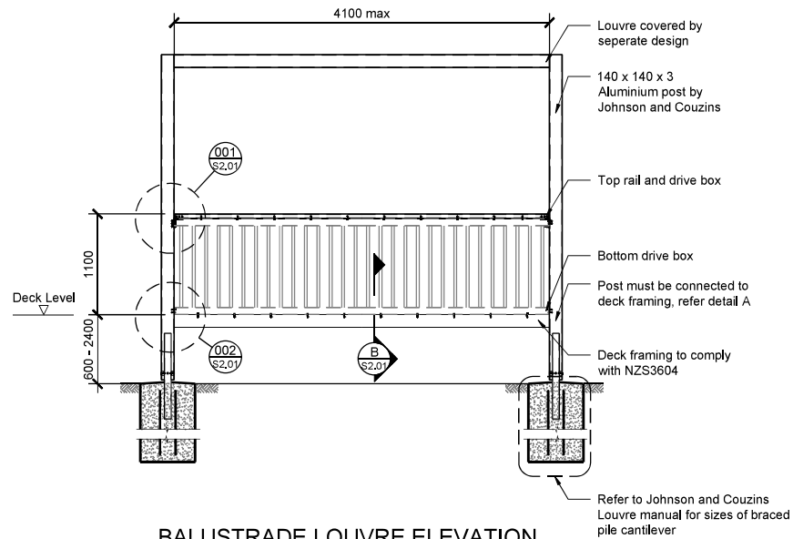
BALUSTRADE LOUVRE ELEVATION SCALE 1:50
