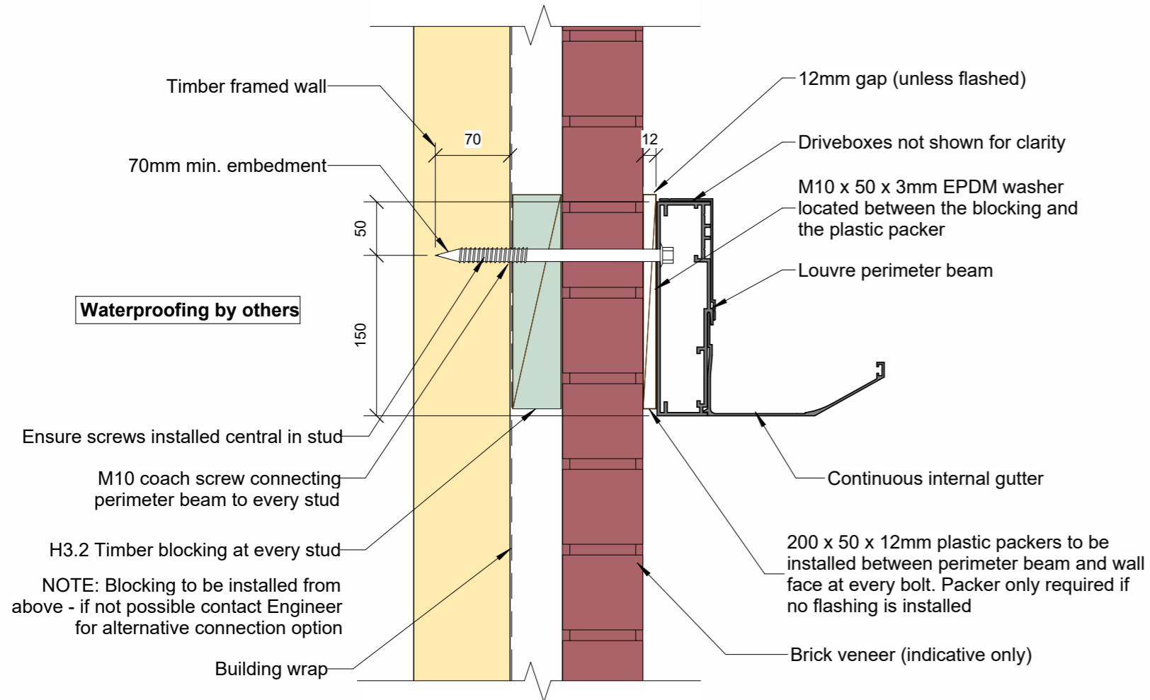
PERIMETER BEAM TO BRICK 1 : 5
